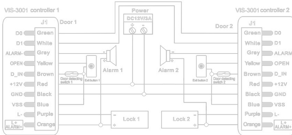
Two VIS-3001 units interconnected & interlocked for 2 doors
