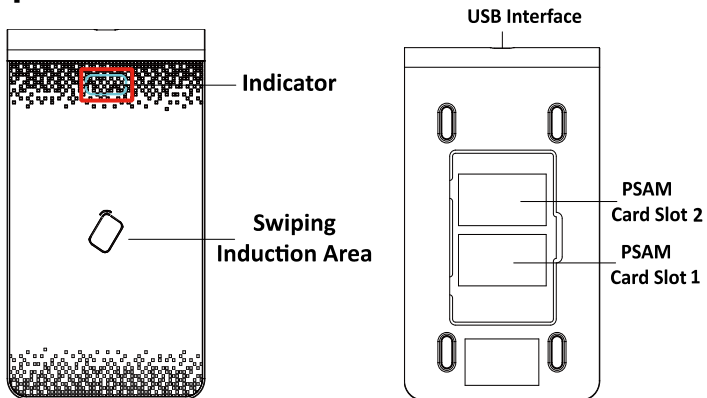
Figure 1-2 Appearance of Card Enrollment Station
